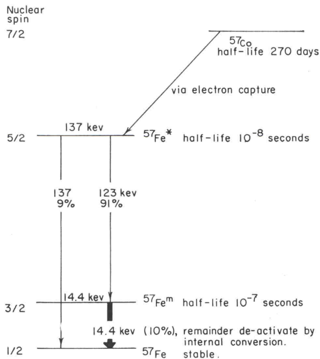
Figure 2. Decay scheme of ^{57}\text{Co} . The shaded transition includes the Mössbauer radiation.
